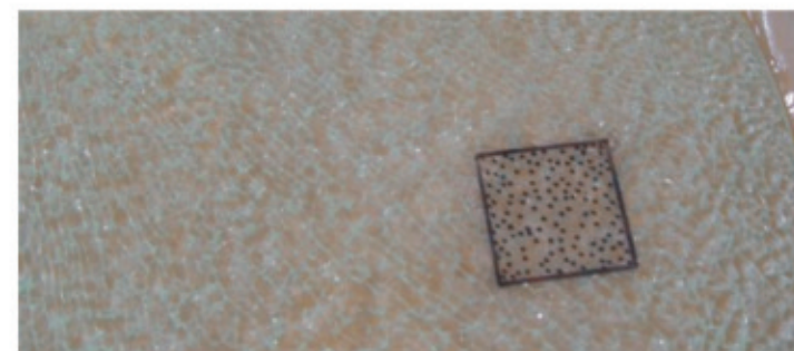
钢化碎片 Fragmentation analysis of toughened glass
